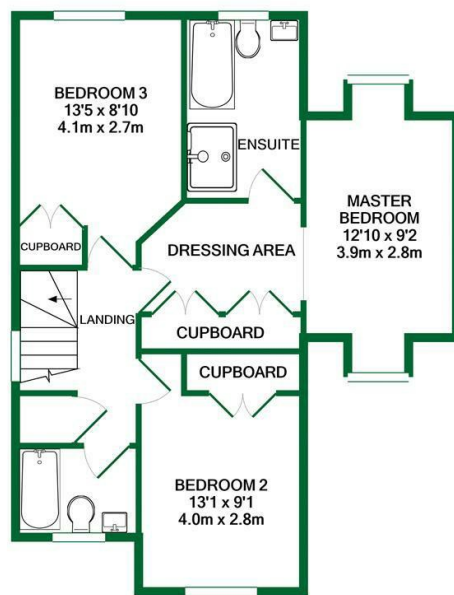
1ST FLOOR
